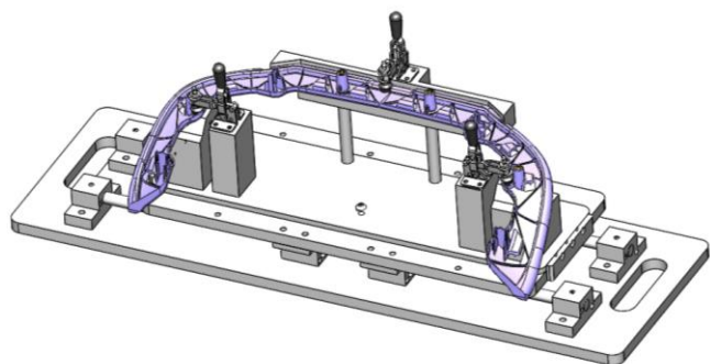
HOLDING FIXTURES WITH SLIDING
